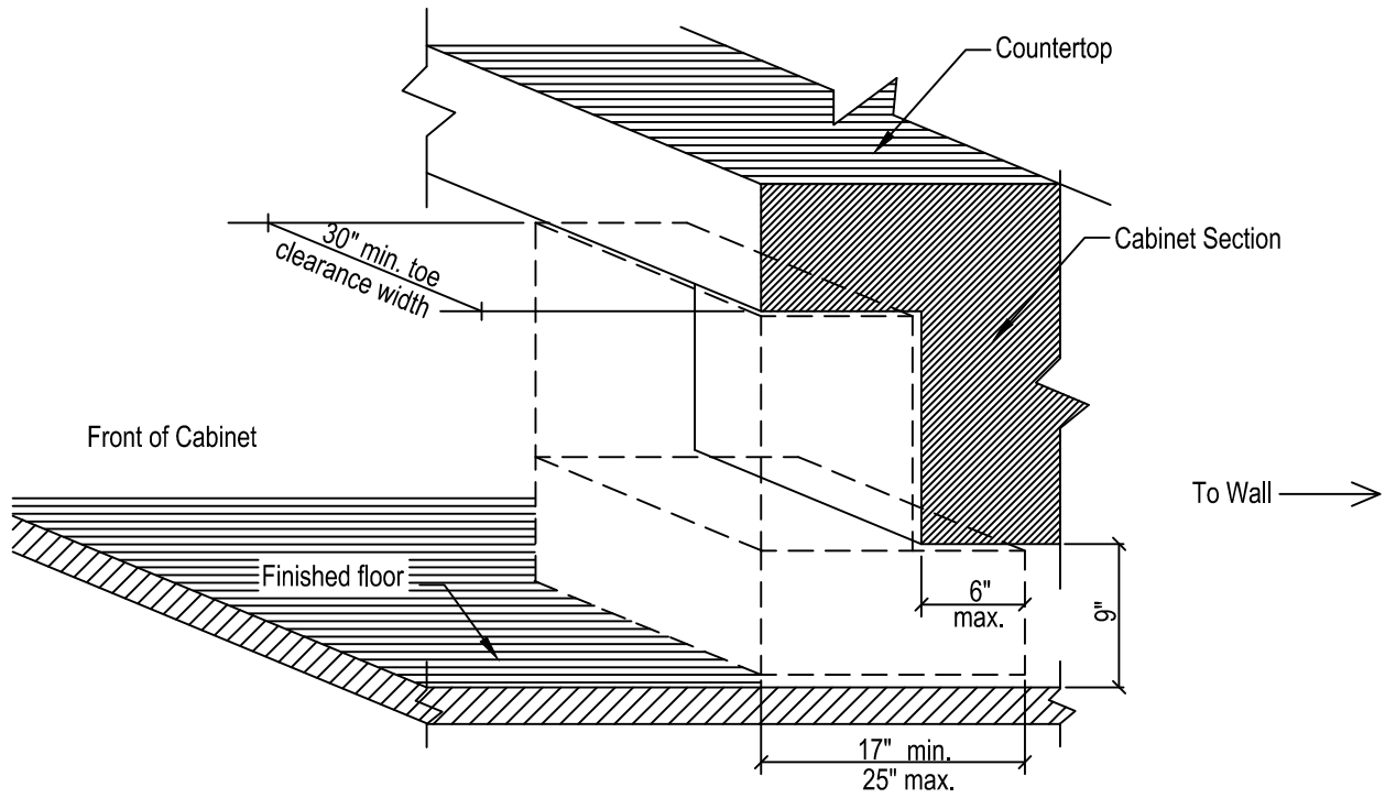
Toe Clearance
