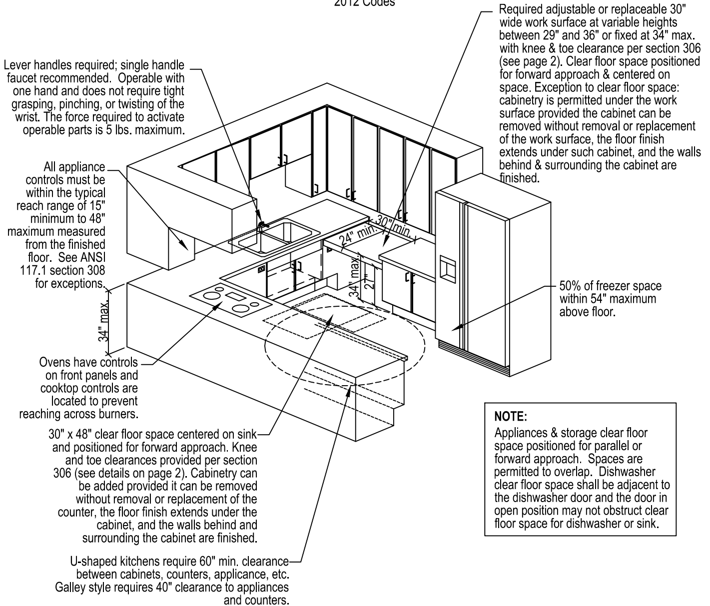
Three-Dimensional Kitchen Layout Diagram
