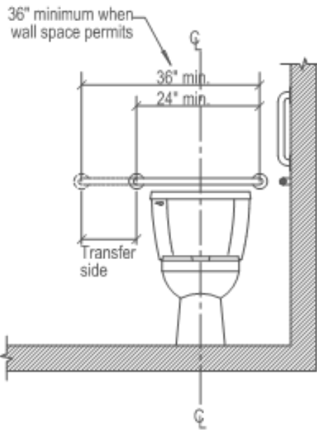
Rear Wall Grab Bar for Water Closet
