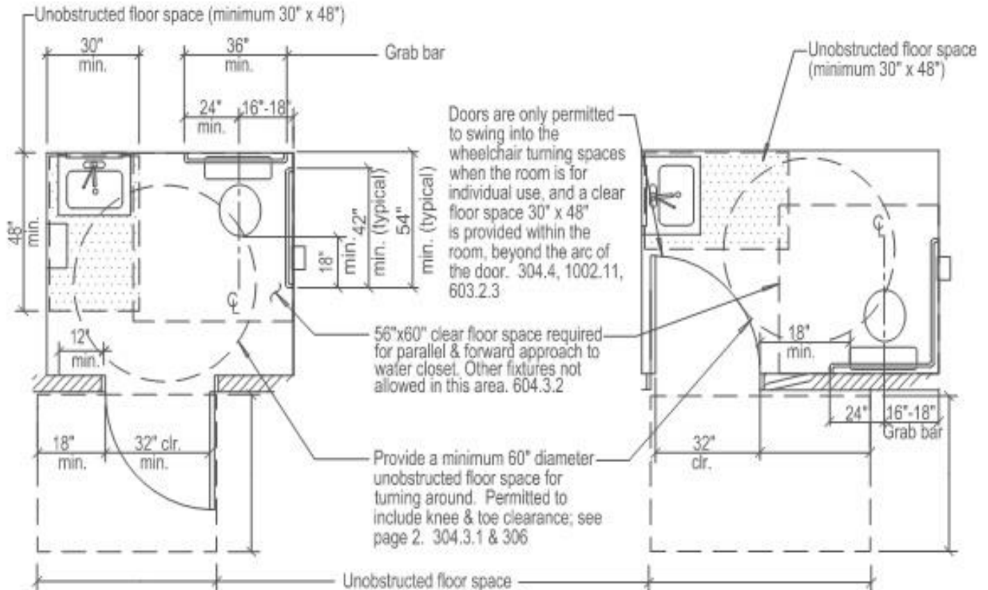
Outward Swinging Door Plan
