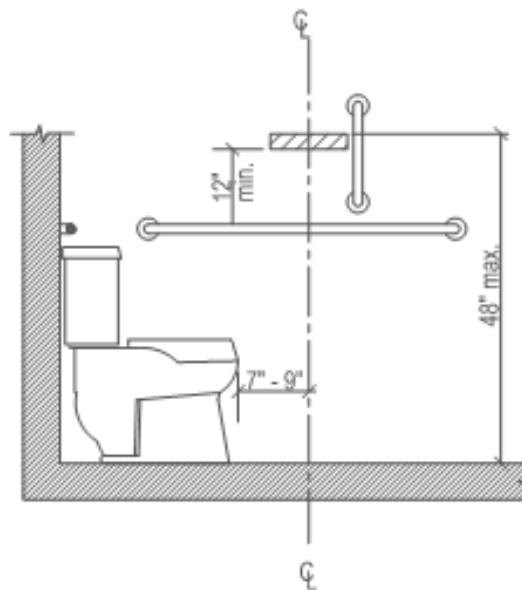
Dispenser Location Above Grab Bar
